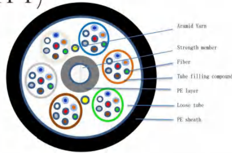
Down Sized Stranded Loose Tube Air-blown Micro Cable (GCYFY) -144B
