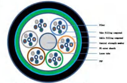
GYTS Outdoor Direct Burial Anti-rat Rodent Single Mode Fiber Optic Cable
