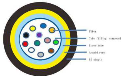
Uni-tube Air-blown Micro Cable (GCYFXTY)
