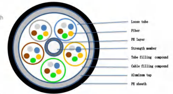
GYTA FTTH Aerial Fiber Optical Cable
