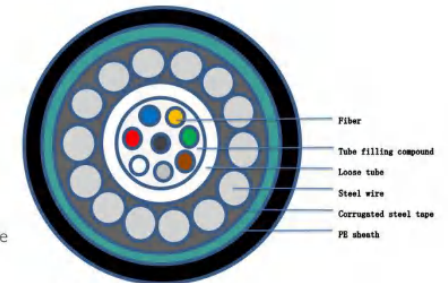
Uni-tube Anti-rodent Optical Cable(GYXTS)
