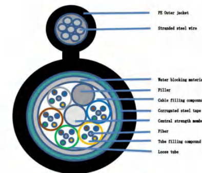
GYTC8S Figure 8 self-supporting aerial cable
