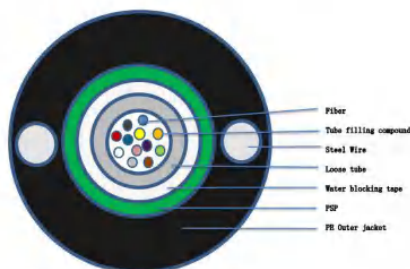
GYXTW Armoured Duct & Aerial fiber optic cable
