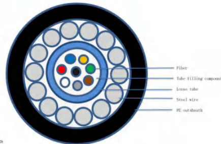
Uni-tube Anti-rodent Optical Cable(GYXTY)
