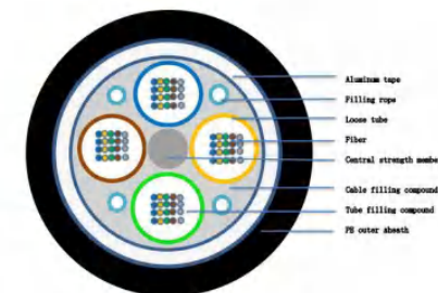
GYDTA layer stranded optical fiber ribbon cable
